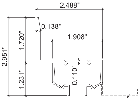
16 NFC100-12 6005-T5 HEAVY DUTY WALL TRACK
