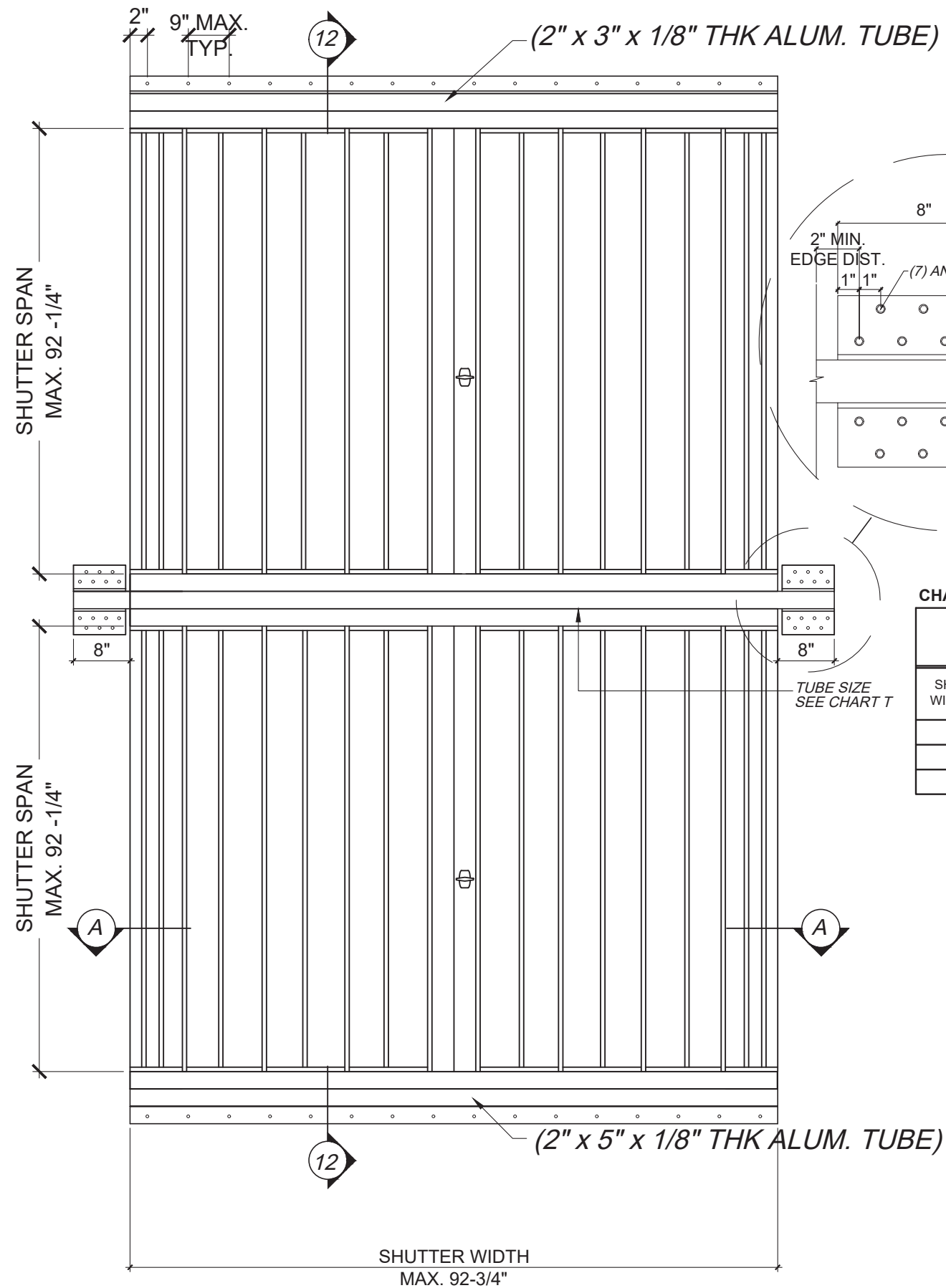
ELEVATION OPTION 1
