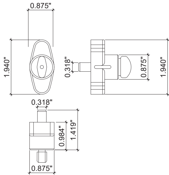
20 EGRESS PUSH LOCK
