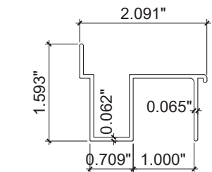
17 NFC100-13 6063-T6 HEAVY DUTY ADJ. TOP SILL
