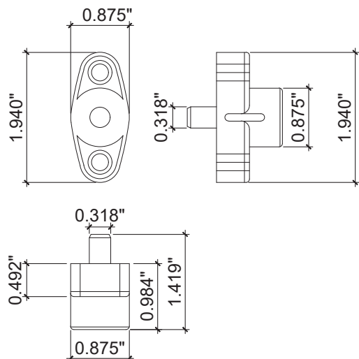
19 PUSH LOCK
