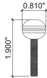
22 THUMB SCREW
