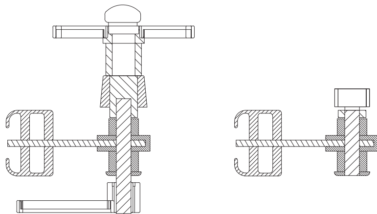
28 EGRESS TURN LOCK OPTION 1 WITH HANDLE
